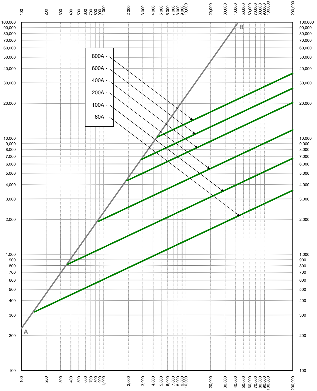
AVAILABLE FAULT CURRENT SYMMETRICAL R.M.S. AMPERES
