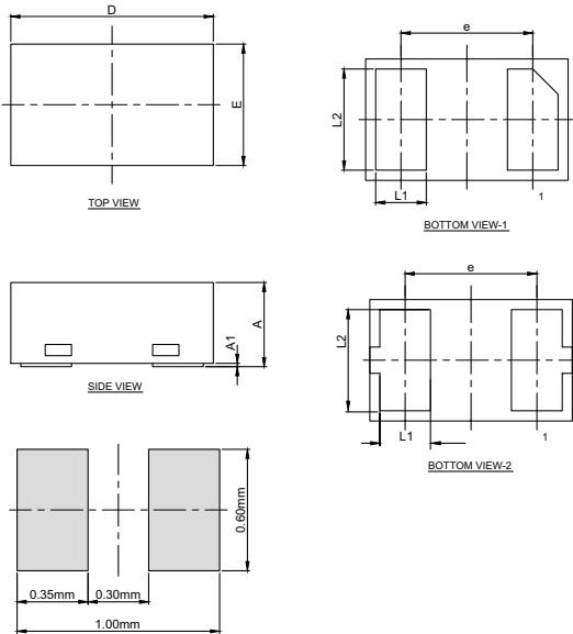
Recommended Soldering Pattern
