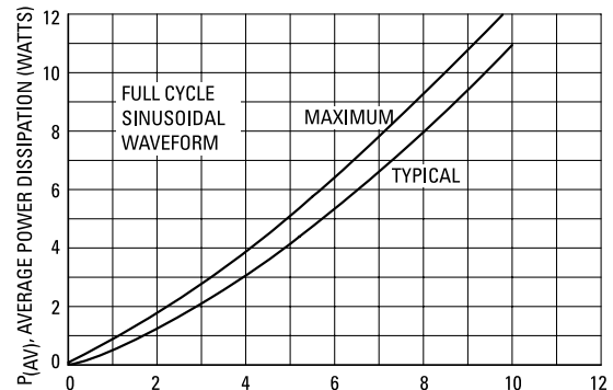
Figure 2. Power Dissipation
