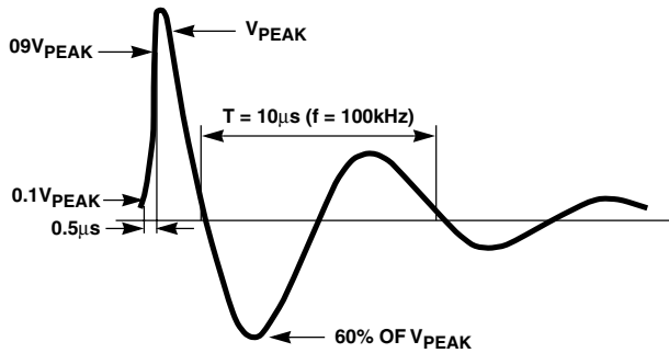
FIGURE 2. THE PROPOSED 0.5μs - 100kHz RING WAVE (OPEN-CIRCUIT VOLTAGE)
