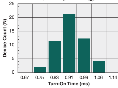
Typical Turn-On Time (N=50, I_L=100mA_{DC} )
