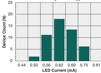
Typical I_L for Switch Dropout (N=50, I_L=100mA_{DC} )
