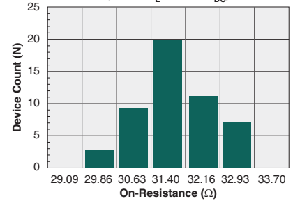
Typical On-Resistance Distribution (N=50, I_L=100mA_{DC} )
