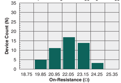
Typical On-Resistance Distribution (N=50, I F =2mA, I L =120mA DC , V L =350V DC )
