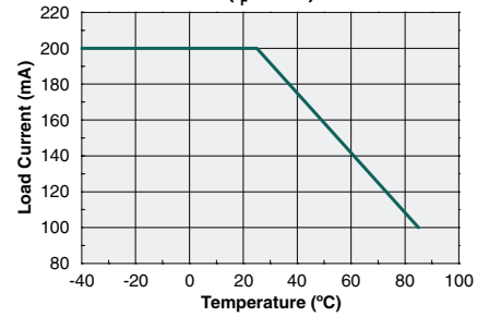
Maximum Load Current vs. Temperature DC-Only Configuration ( I_F=2\text{mA} )
