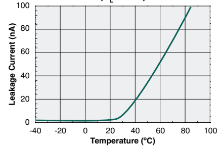
Typical Leakage vs. Temperature ( V_L=600\text{V} )
