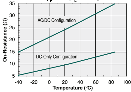
Typical On-Resistance vs. Temperature ( I_F=5mA, I_L=60mA )
