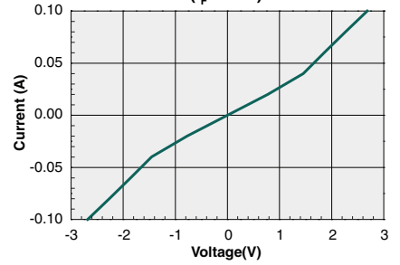
Typical Load Current vs. Load Voltage AC/DC Configuration ( I_F=5mA )
