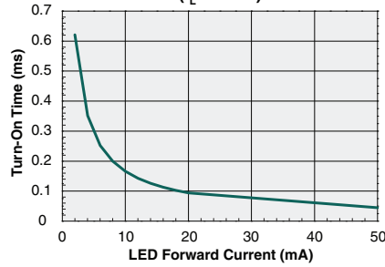
Typical Turn-On Time vs. LED Forward Current ( I_L=30mA )
