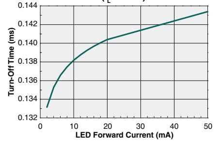
Typical Turn-Off Time vs. LED Forward Current ( I_L=30mA )
