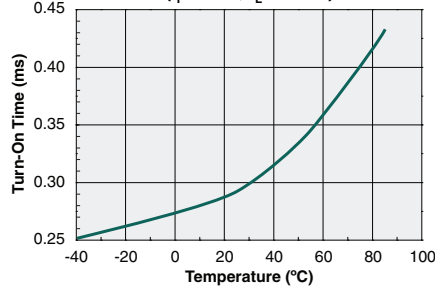
Typical Turn-On Time vs. Temperature ( I_F=5mA , I_L=80mA )
