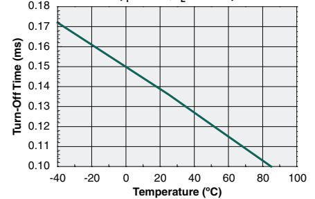
Typical Turn-Off Time vs. Temperature ( I_F=5mA , I_L=80mA )
