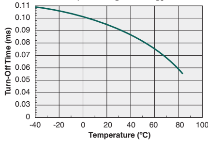
Typical Turn-Off Time vs. Temperature ( I_F=5\text{mA} , I_L=200\text{mA}_{\text{DC}} )
