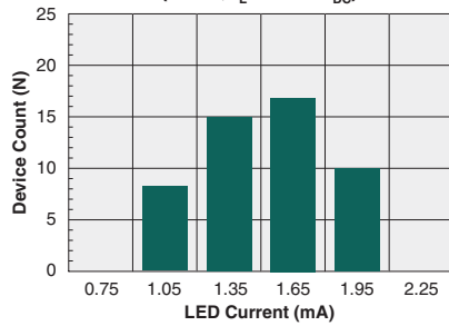
Typical I_F for Switch Operation (N=50, I_L=350mA_{DC} )
