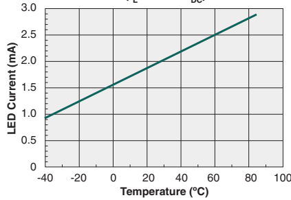
Typical I_F for Switch Dropout vs. Temperature ( I_L=200\text{mA}_{\text{DC}} )
