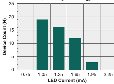
Typical I_F for Switch Dropout (N=50, I_L=350mA_{DC} )
