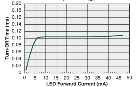
Typical Turn-Off Time vs. LED Forward Current ( I_L=200mA_{DC} )
