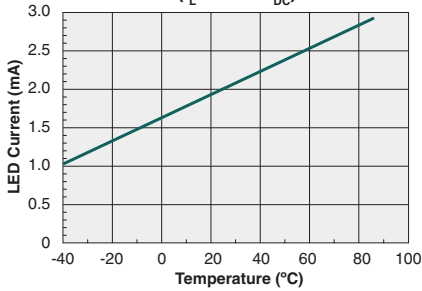
Typical I_F for Switch Operation vs. Temperature ( I_L=200\text{mA}_{\text{DC}} )
