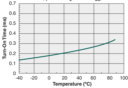
Typical Turn-On Time vs. Temperature ( I_F=5\text{mA} , I_L=200\text{mA}_{\text{DC}} )
