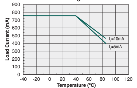
Maximum Load Current vs. Temperature DC Configuration
