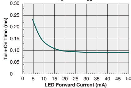
Typical Turn-On Time vs. LED Forward Current ( I_L=200mA_{DC} )
