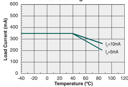
Maximum Load Current vs. Temperature AC/DC Configuration
