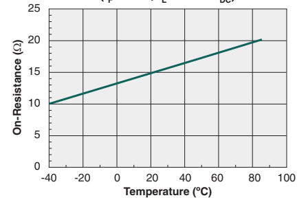
Typical On-Resistance vs. Temperature ( I_F=5\text{mA} , I_L=150\text{mA}_{DC} )
