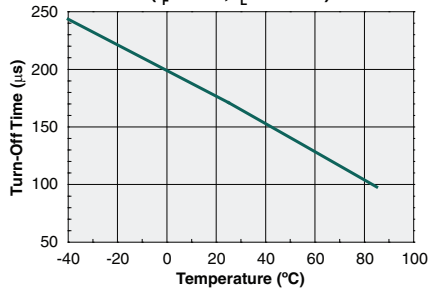
Typical Turn-Off Time vs. Temperature ( I_F=5mA, I_L=100mA )
