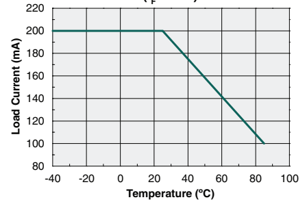
Maximum Load Current vs. Temperature ( I_F=3mA )
