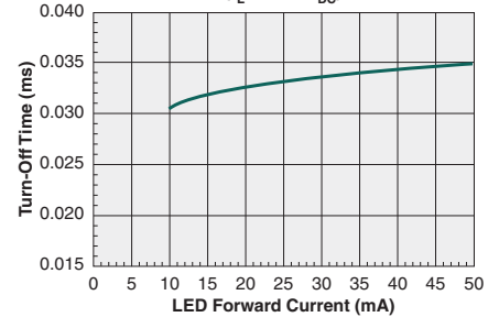
Typical Turn-Off Time vs. LED Forward Current ( I_L=50\text{mA}_{DC} )
