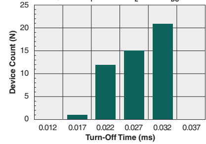
Typical Turn-Off Time (N=50, I_F=10\text{mA} , I_L=50\text{mA}_{DC} )
