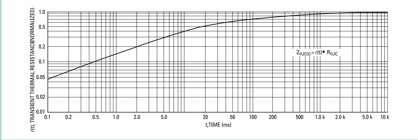
Figure 10. Thermal Response
