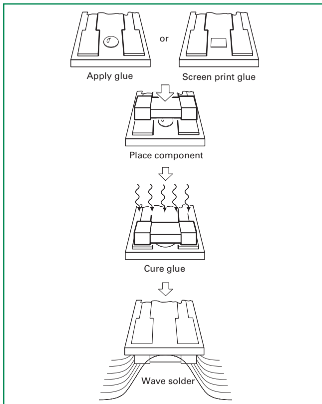
Figure AN1005.6 Wave Soldering PCBs With Surface Mount Components Only
