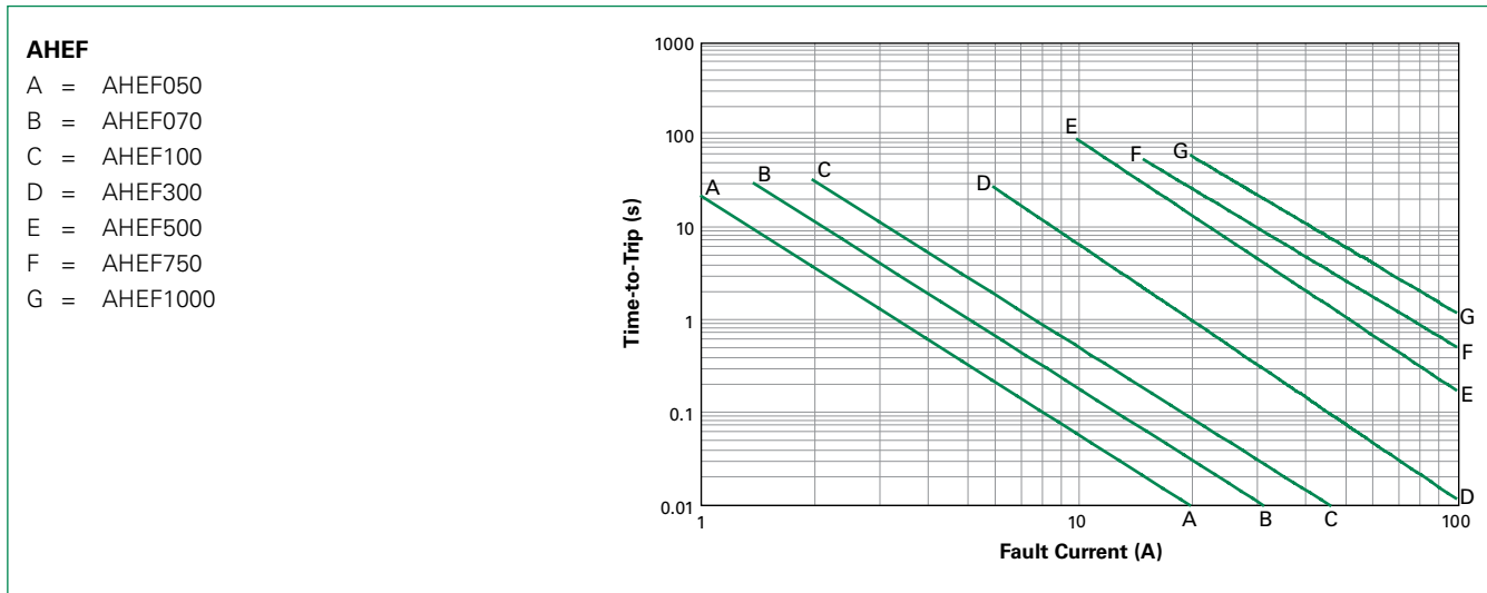
Typical Time-to-Trip Curves at 25°C
