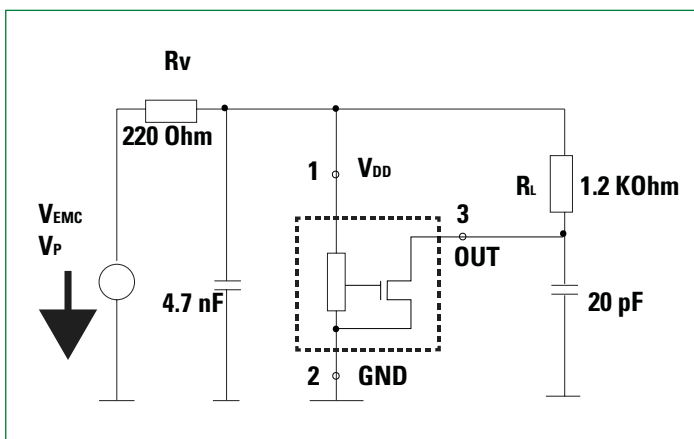
Figure 3. 3-Wire Devices
