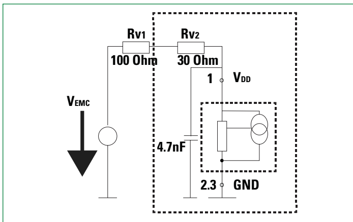
Figure 4. 2-Wire Device
