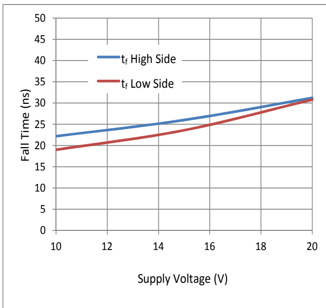
Figure 11. Fall Time vs. Supply Voltage
