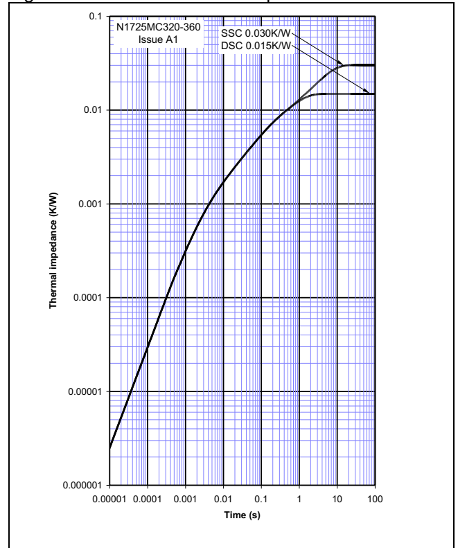
Figure 2 – Transient thermal impedance
