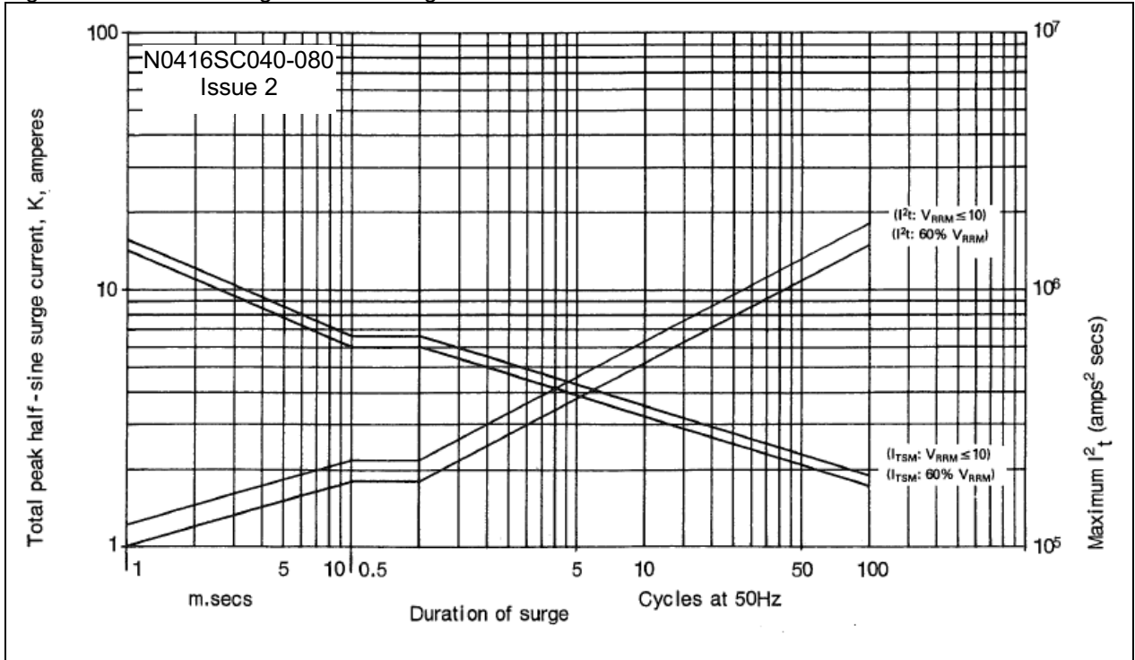
Figure 7 - Maximum surge and I 2 t Ratings at initial T J – 125°C
