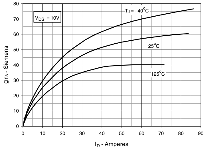
Fig. 8. Transconductance
