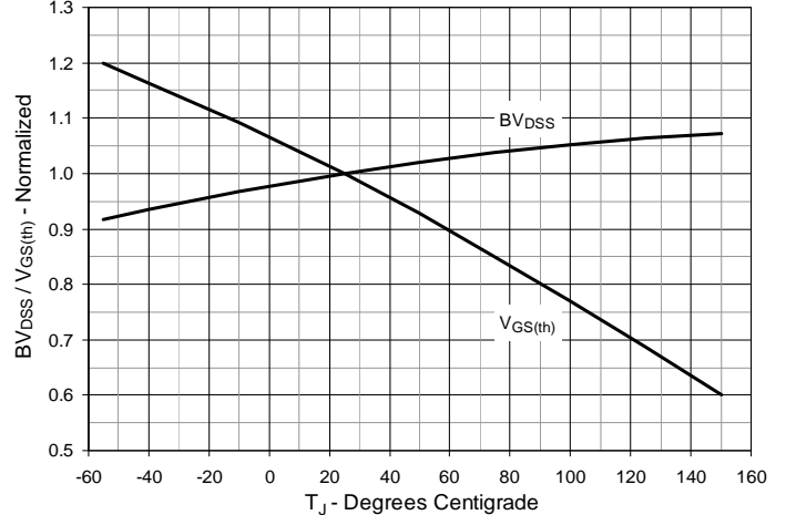
Fig. 6. Normalized Breakdown & Threshold Voltages vs. Junction Temperature
