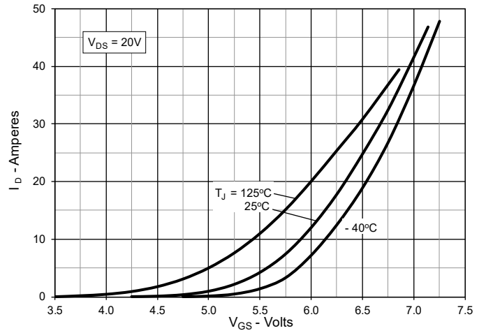
Fig. 8. Input Admittance
