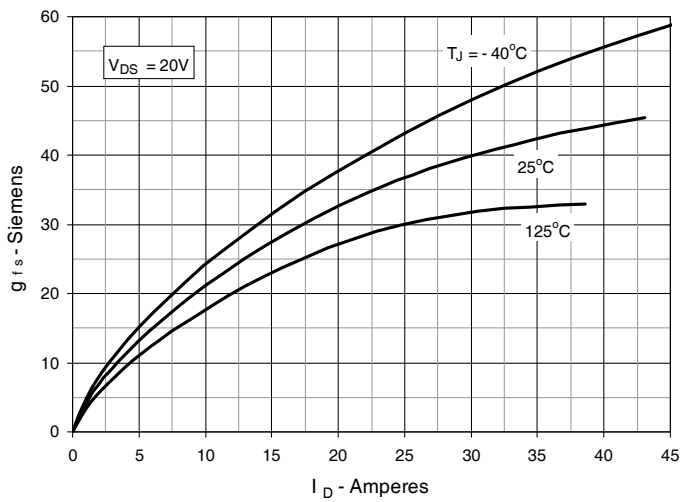
Fig. 9. Transconductance
