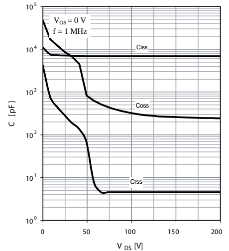
Fig. 9 Typ. capacitances
