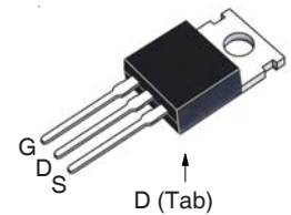
TO-220 (IXTP)
