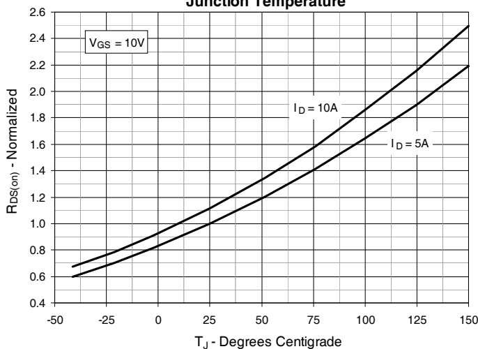
Fig. 4. R_{DS(on)} Normalized to I_D = 5\text{A} Value vs. Junction Temperature
