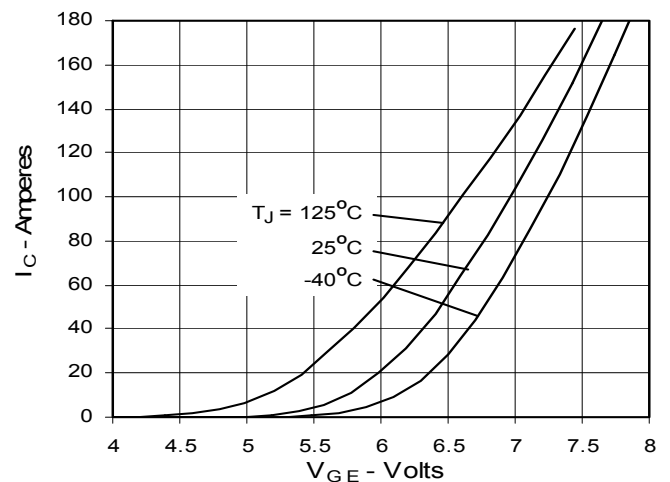
Fig. 6. Input Admittance
