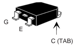
PLUS220SMD (IXGV...S)
