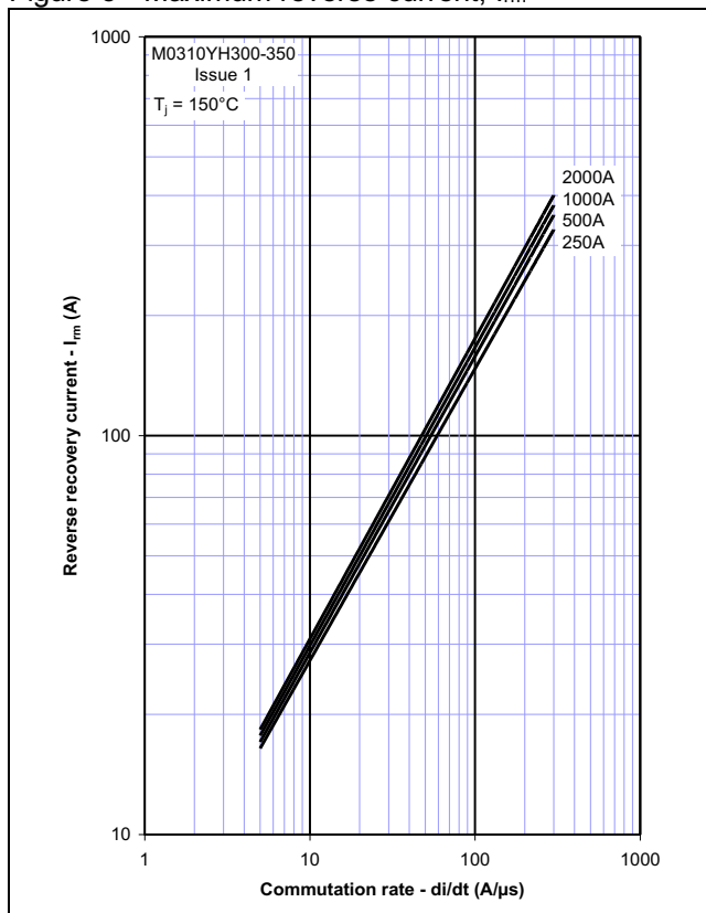
Figure 5 - Maximum reverse current, I_{rm}
