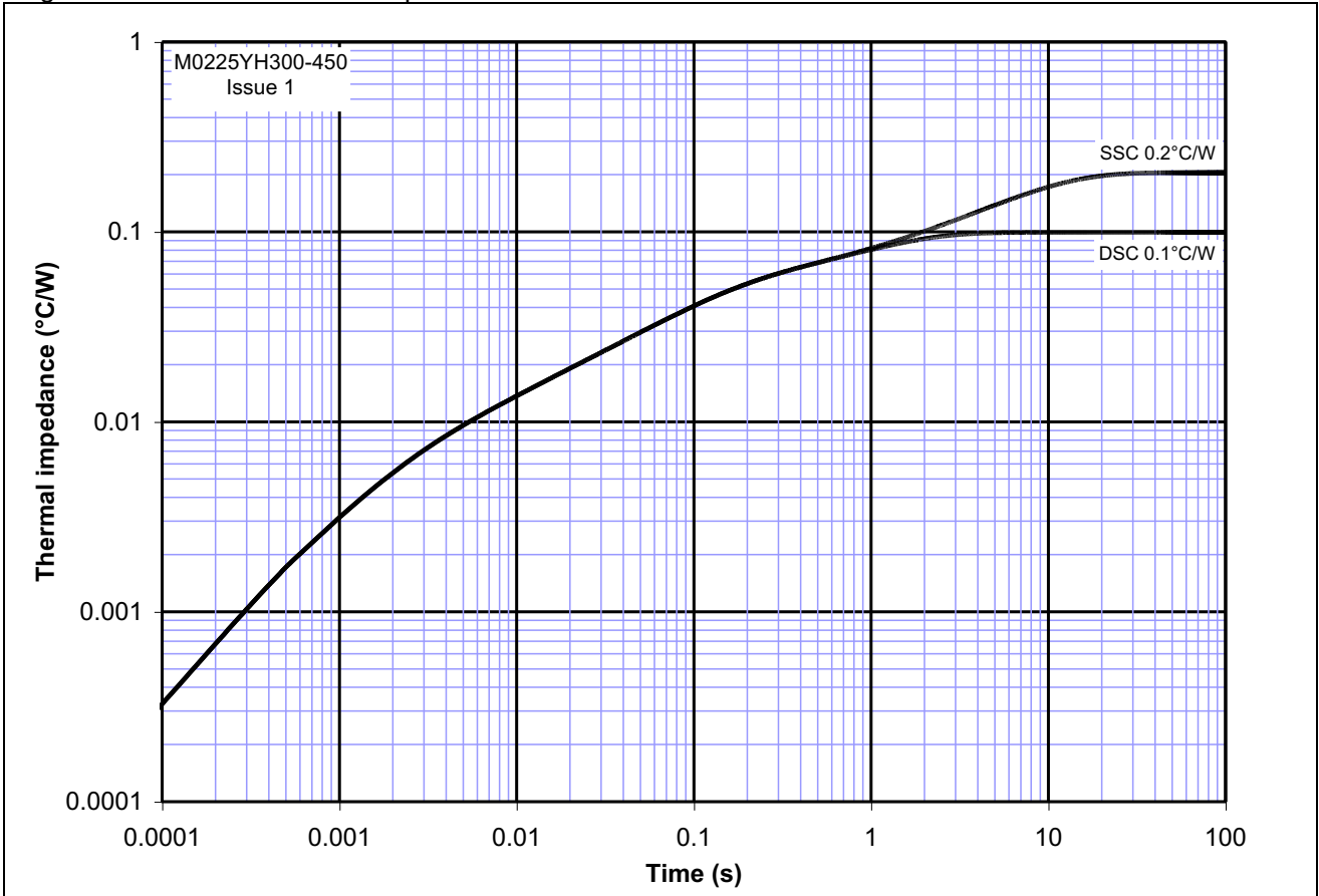
Figure 18 – Transient thermal impedance
