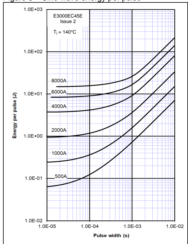
Figure 8 – Sine wave energy per pulse
