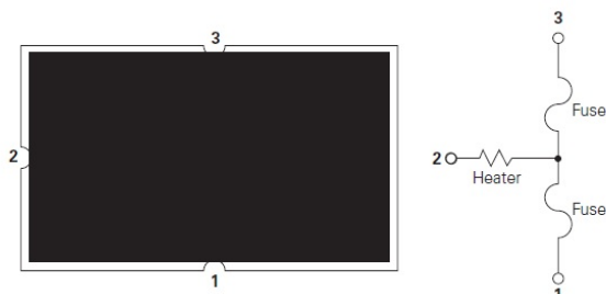
Device Circuit:
