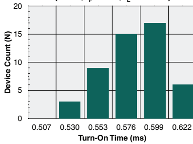
Typical Turn-On Time (N=50, I_f=5mA , I_L=100mA )
