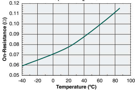
Typical On-Resistance vs. Temperature ( I_F=2mA, I_L=1A )
