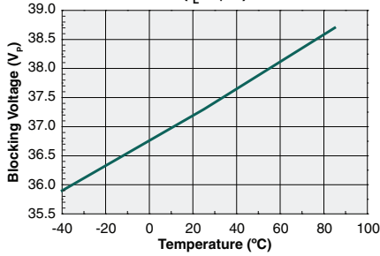
Typical Blocking Voltage vs. Temperature ( I_L=1\mu A )
