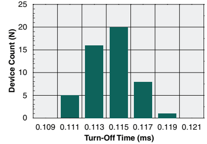
Typical Turn-Off Time Distribution (N=50, I_F=5mA , I_L=100mA )
