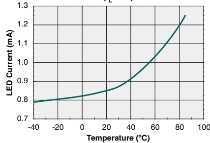
LED Current to Operate vs. Temperature ( I_L=1A )
