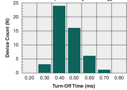
Typical Turn-Off Time (N=50, I_F=10\text{mA} , I_L=120\text{mA}_{DC} )
