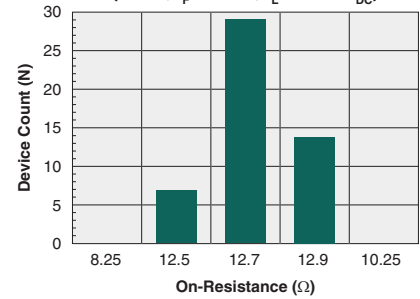
Typical On-Resistance Distribution (N=50, I_F=10\text{mA} , I_L=120\text{mA}_{DC} )
