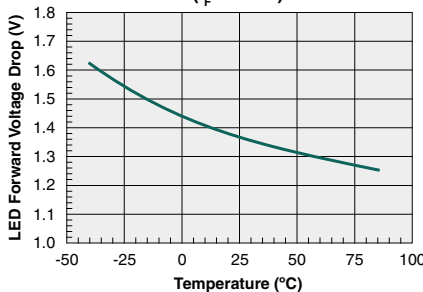
Typical LED Forward Voltage Drop vs. Temperature ( I_F=10\text{mA} )
