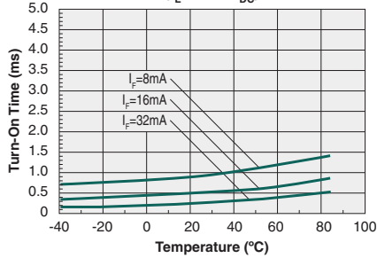
Typical Turn-On Time vs. Temperature ( I_L=40mA_{DC} )
