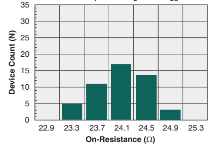
Typical On-Resistance Distribution (N=50, I_F=8\text{mA} , I_L=85\text{mA}_{DC} )
