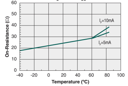
Typical Steady State On-Resistance vs. Temperature ( I_L=120\text{mA}_{DC} )
