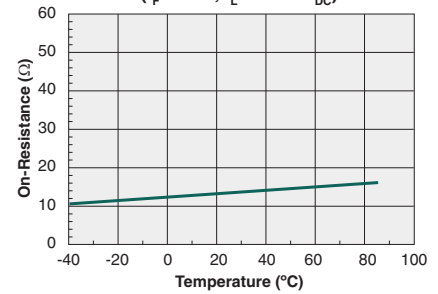
Typical On-Resistance vs. Temperature ( I_F=0\text{mA} , I_L=170\text{mA}_{DC} )
