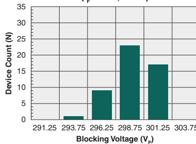
Typical Blocking Voltage Distribution (I F =5mA, N=50)
