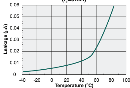
Typical Leakage vs. Temperature Measured Across Pins 7&8 ( I_F=5mA )
