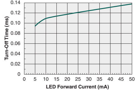
Typical Turn-Off Time vs. LED Forward Current ( I_L=170\text{mA}_{DC} )
