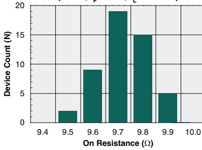
Typical On-Resistance Distribution (N=50, I_F=5mA , I_L=120mA )
