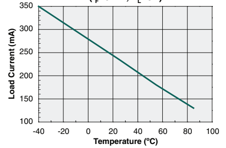
Typical Current Limiting vs. Temperature ( I_F=5mA, V_L=8V )
