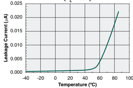
Typical Leakage vs. Temperature Measured Across Pins 5&6, 7&8 ( V_L=250V )
