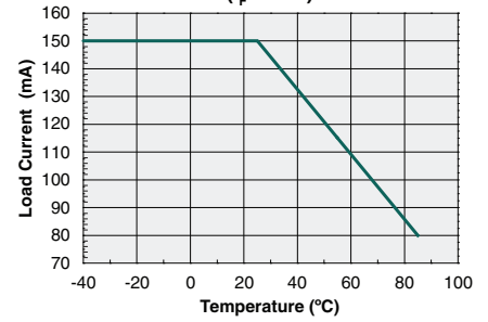
Typical Current Limiting vs. Temperature ( I_F=5mA, V_L=8V )
