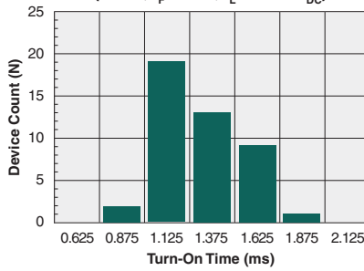
Typical Turn-On Time (N=50, I_F=5mA , I_L=170mA_{DC} )
