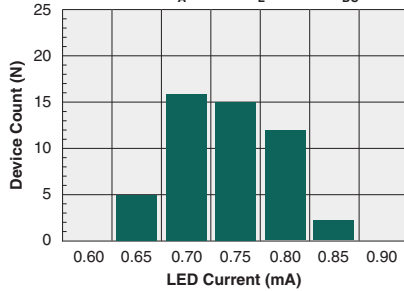
Typical I_F for Switch Operation (N=50, T_A=25^\circ C , I_L=120mA_{DC} )
