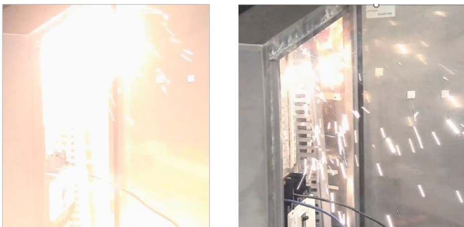
FIGURE 9. A short circuit on a dc bus with 1000 A maximum current.
