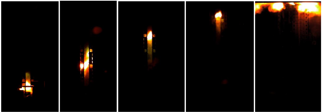
FIGURE 10. Freeze frames from high-speed video with light filter showing short circuit on dc bus with a 1000 A maximum current.
