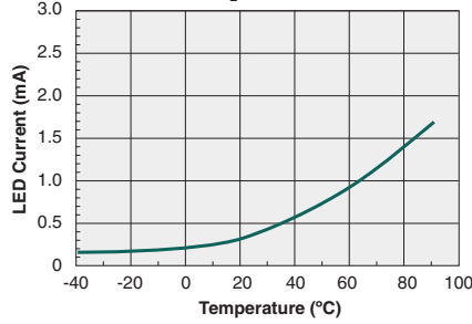
Typical I_F for Switch Operation vs. Ambient Temperature ( I_L=80\text{mA} )
